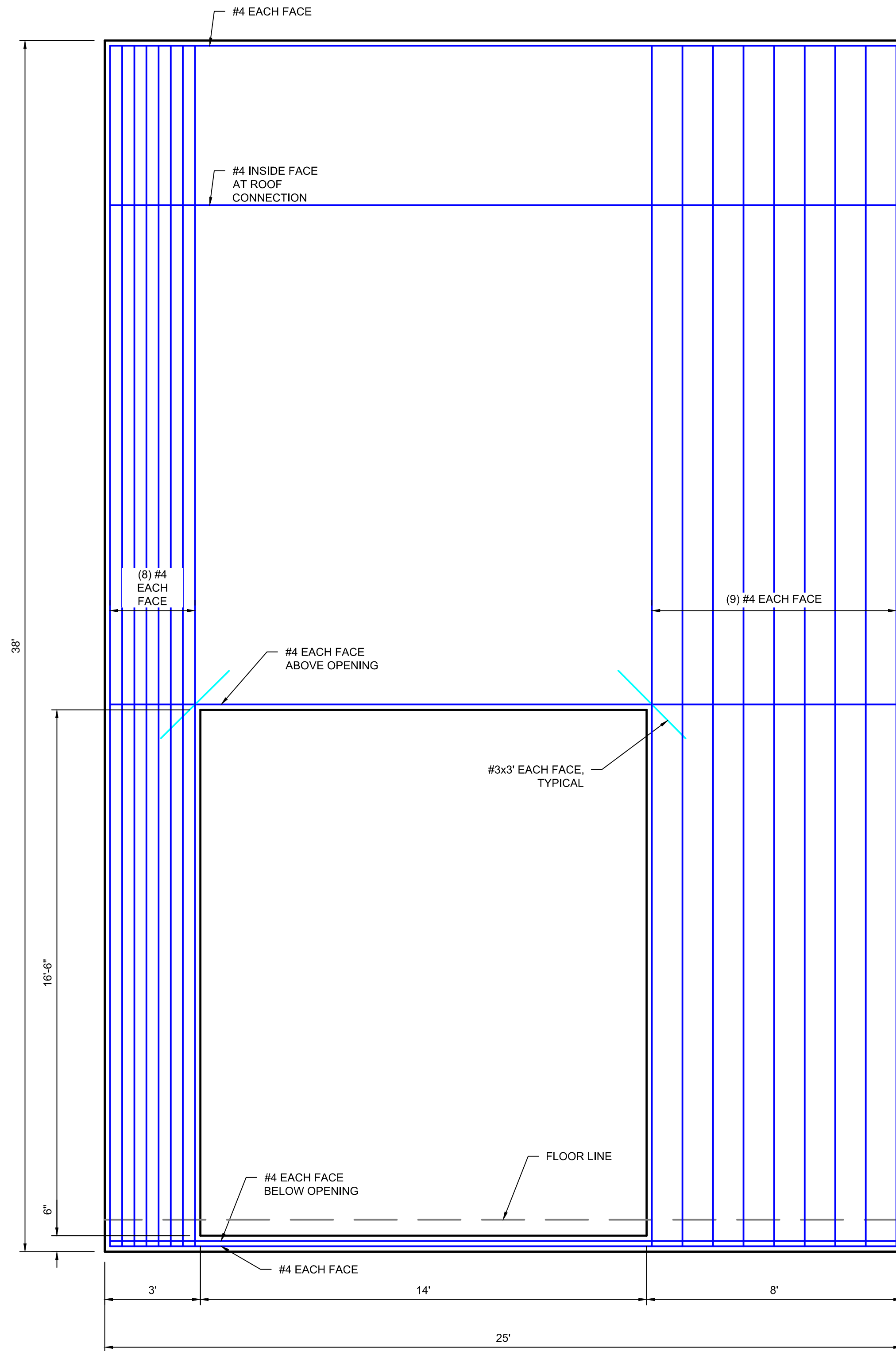
TIPS REINFORCING 3/8" = 1'-0"
