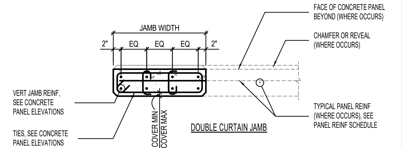
TYPICAL DOUBLE CURTAIN JAMB SCALE: NTS
