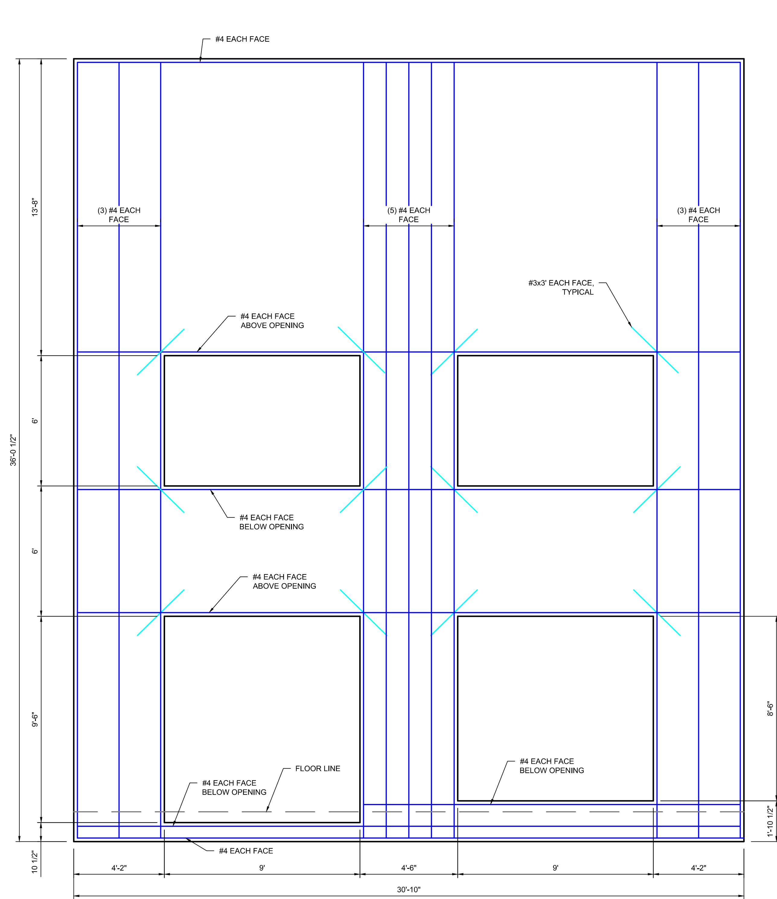
TIPS REINFORCING 3/8" = 1'-0"
